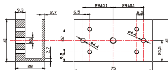
U Bracket Installation
